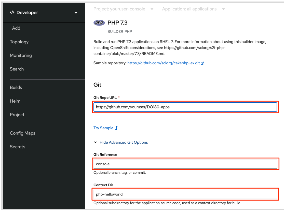
Figure 6.20: Setting Advanced Git Options for the application
