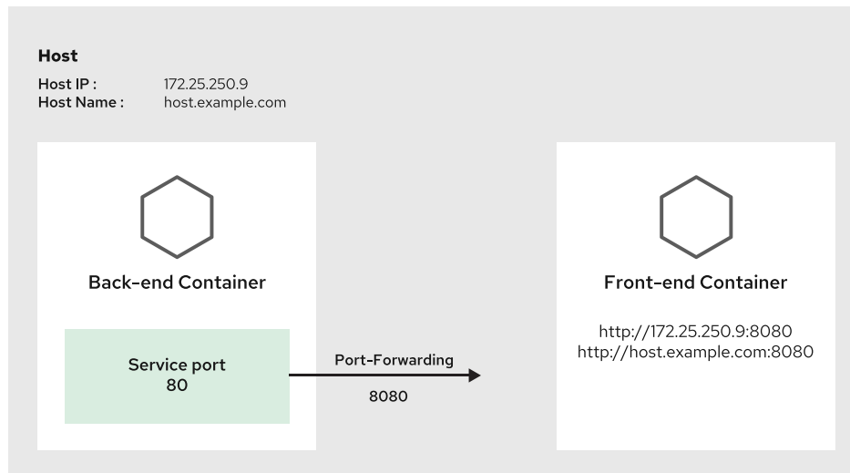
Figure 7.2: Multi-Container Applications for rootless containers
