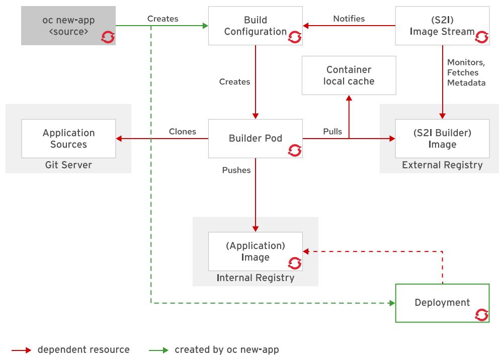
Figure 6.8: Deployment and dependent resources
