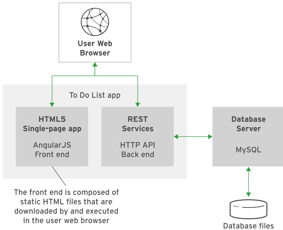
Figure 7.3: To Do List application logical architecture
