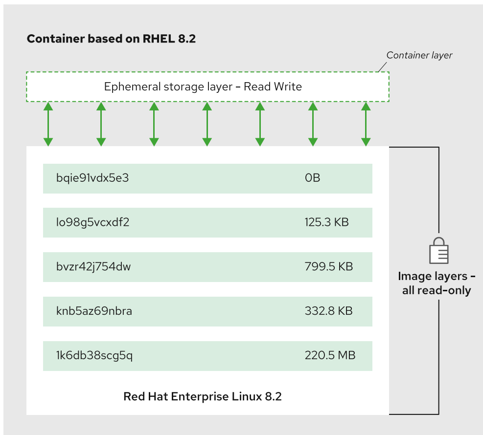
Figure 3.3: Container layers
