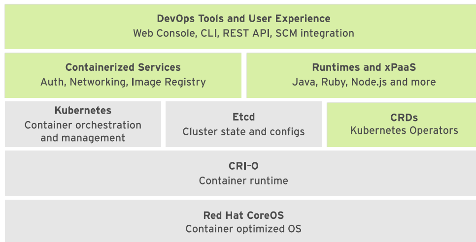
Figure 6.1: OpenShift component stack
