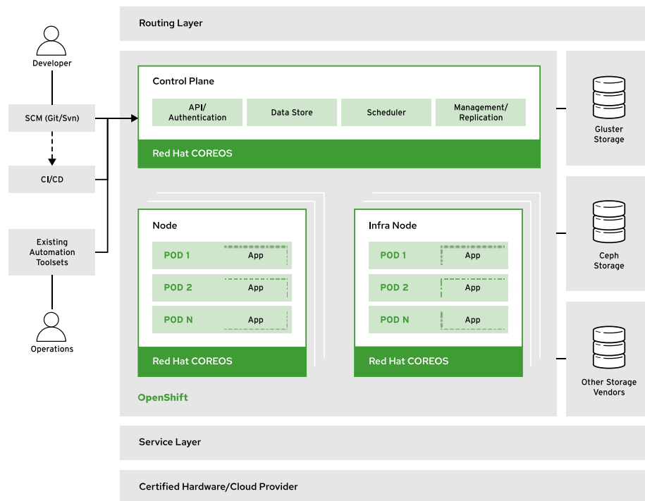
Figure 6.2: OpenShift and Kubernetes architecture
